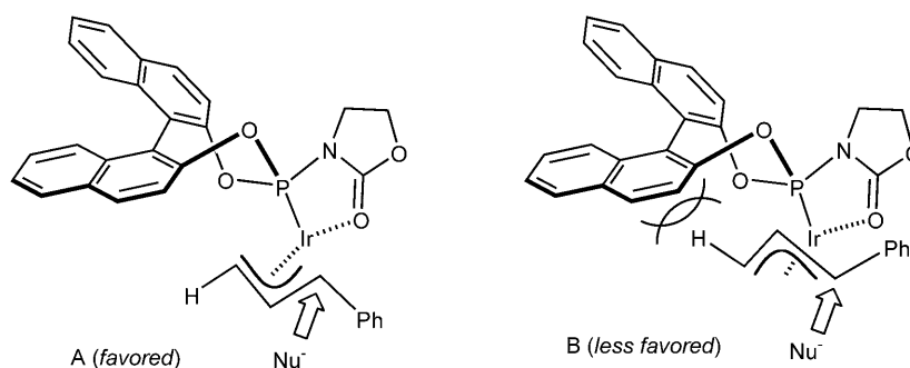
Figure 5. Two plausible transition states of the nucleophilic attack to \pi -allyliridium intermediates.
