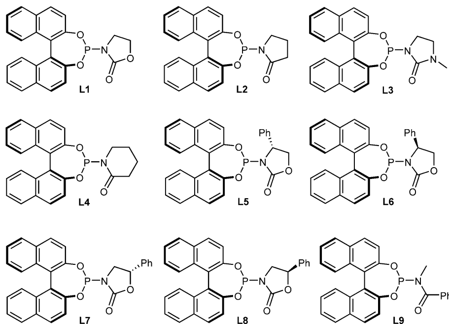
Figure 2. Newly prepared chiral phosphoramidite ligands.
