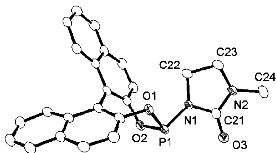
Figure 4. ORTEP drawing of L3 . Hydrogen atoms are omitted for clarity. Thermal ellipsoids are drawn at 50% probability. Selected bond lengths (Å), angles (deg), and torsion angles (deg): P1–O1, 1.6537(11); P1–O2, 1.6394(12); P1–N1, 1.6768(13); O1–P1–O2, 99.00(6); O1–P1–N1, 94.27(7); O2–P1–N1, 105.47(7); P1–N1–C21, 119.82(11); P1–N1–C22, 130.21(11); C21–N1–C22, 109.68(12); N1–C21–N2, 108.10(14); N1–C21–O3, 125.03(15); N2–C21–O3, 126.86(16); P1–N1–C21–O3, 10.5(2).
