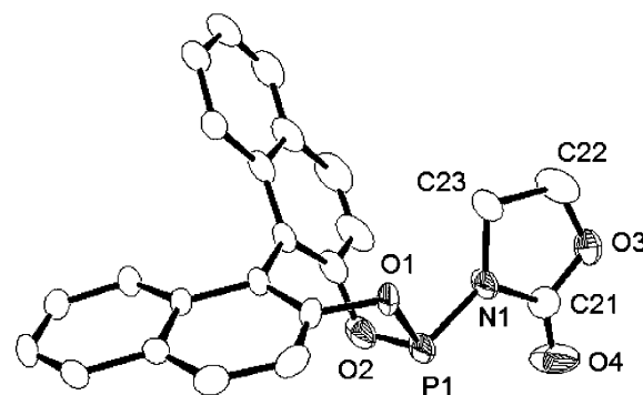
Figure 3. ORTEP drawing of L1 . Hydrogen atoms are omitted for clarity. Thermal ellipsoids are drawn at 50% probability. Selected bond lengths (Å), angles (deg), and torsion angles (deg): P1–O1, 1.654(3); P1–O2, 1.617(5); P1–N1, 1.715(4); O1–P1–O2, 99.76(17); O1–P1–N1, 92.57(19); O2–P1–N1, 102.7(2); P1–N1–C21, 120.2(3); P1–N1–C23, 128.9(3); C21–N1–C23, 110.6(4); N1–C21–O3, 110.2(5); N1–C21–O4, 126.2(5); O3–C21–O4, 123.5(5); P1–N1–C21–O4, 9.9(13).
